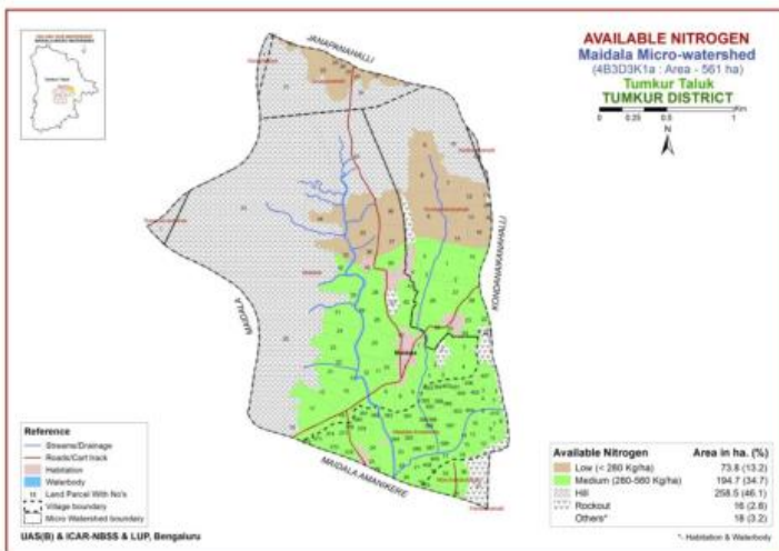
Soil fertility map
